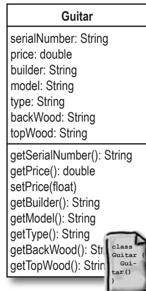
Guitar.java
